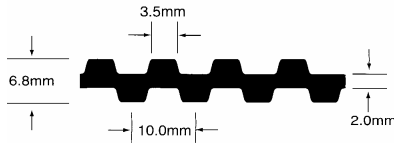
Nominal Dimensions
